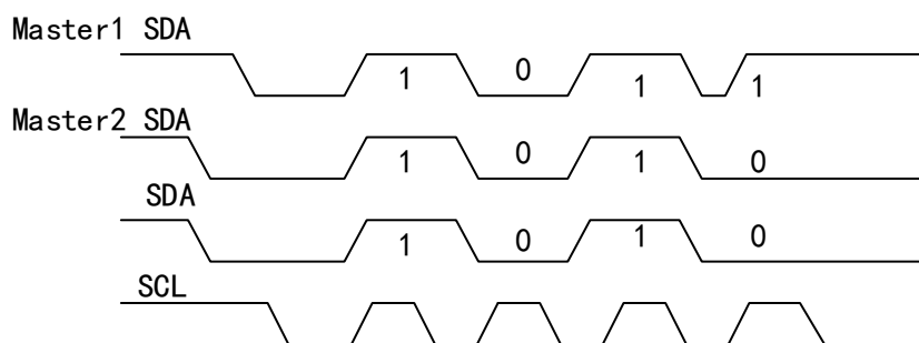
Figure 81 SDA Timing Diagram
