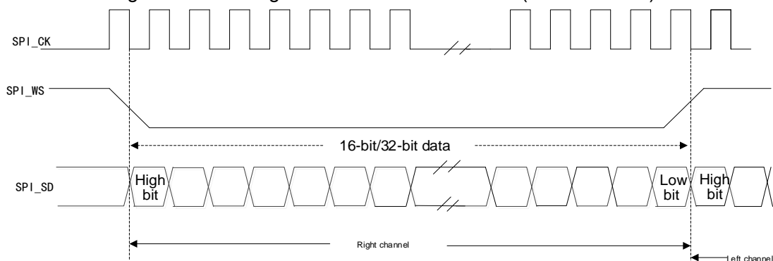
Figure 89 MSB Alignment Standard Waveform (16/32-bit data)
